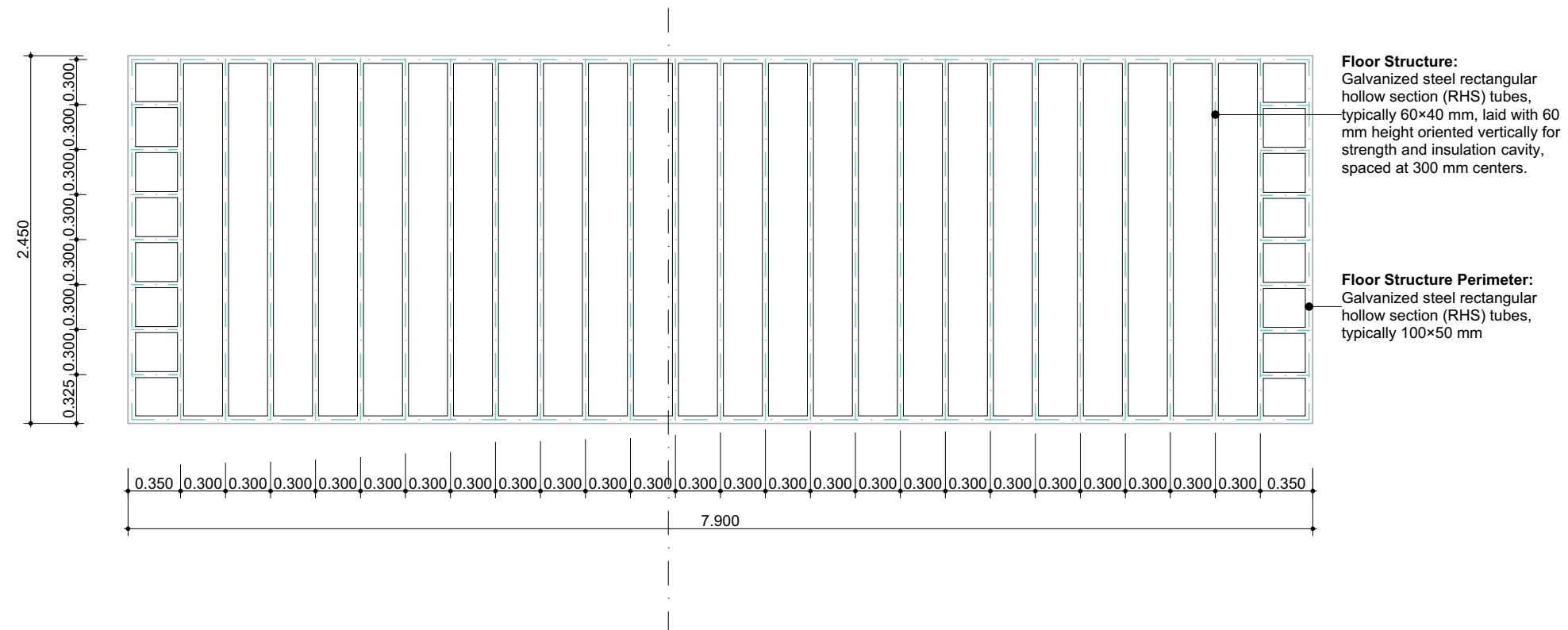
-1. BASE DRAWING 1:40
