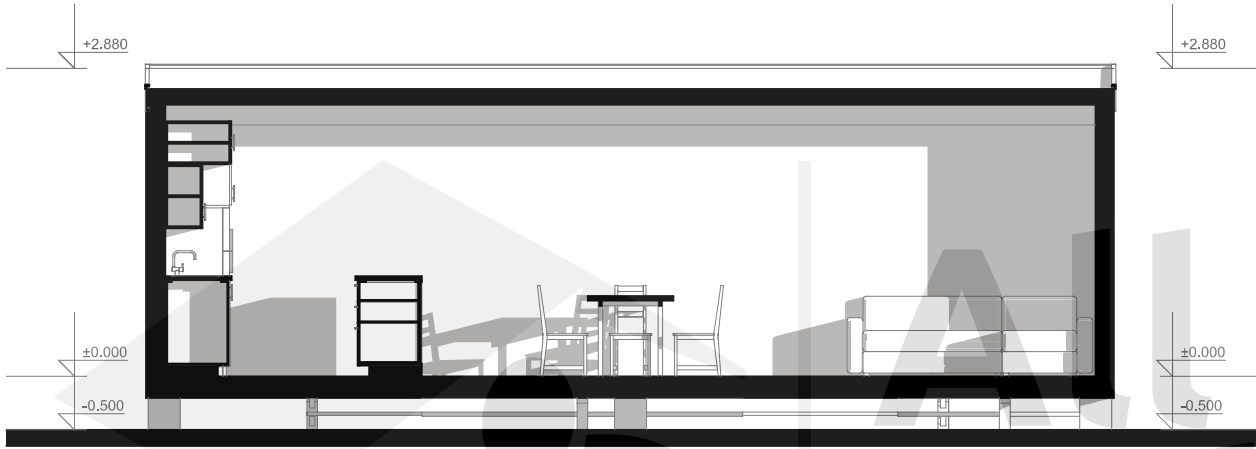
SECTION 16-16
